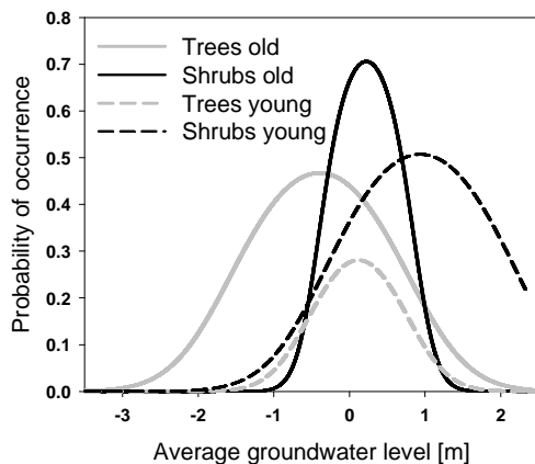
Figure 1. Probability of occurrence for the different species groups along a gradient of increasing AWL
