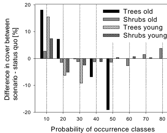
Figure 2. Differences in cover of probability of occurrence classes between climate change scenario and calculated status quo
